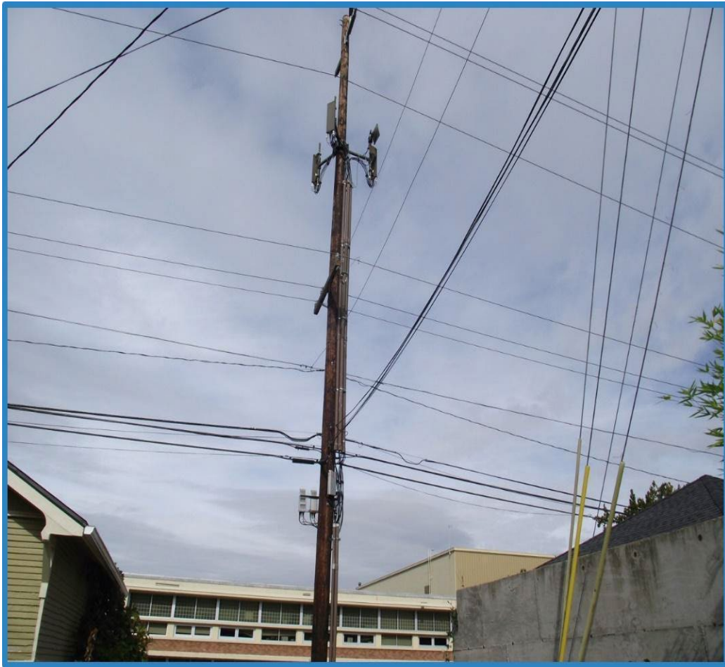
Figure 9.5 - Joint Use W-Arrows
